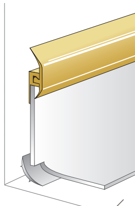
Capping strip - Clip system
